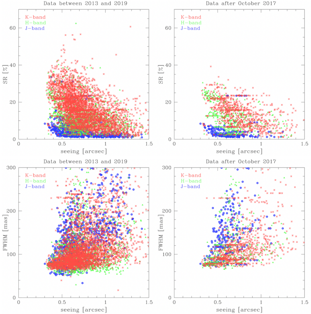
Figure 7: GeMS performance, overall on left and post Toptica upgrade on right
