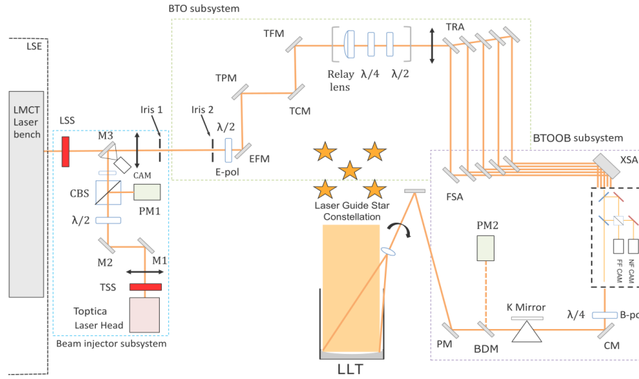
Figure 3: Block diagram of BTO with both laser systems shown. Figure from Chirre et al. (2018) [11]
